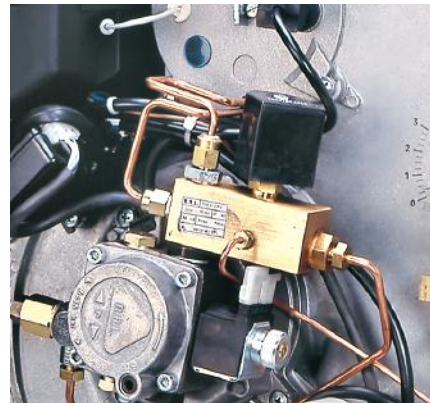
Fuel pump (RG5D)
