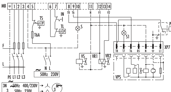
GAS 5 - 6 With seal control
