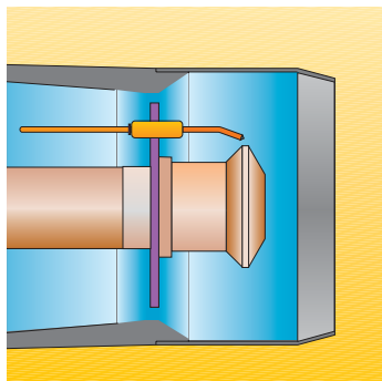
Example of a GAS burner combustion head
