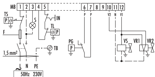
GAS 3 - 4 Without seal control
