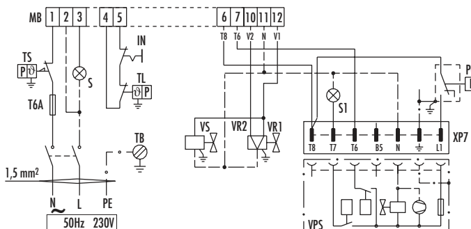
GAS 3 - 4 With seal control
